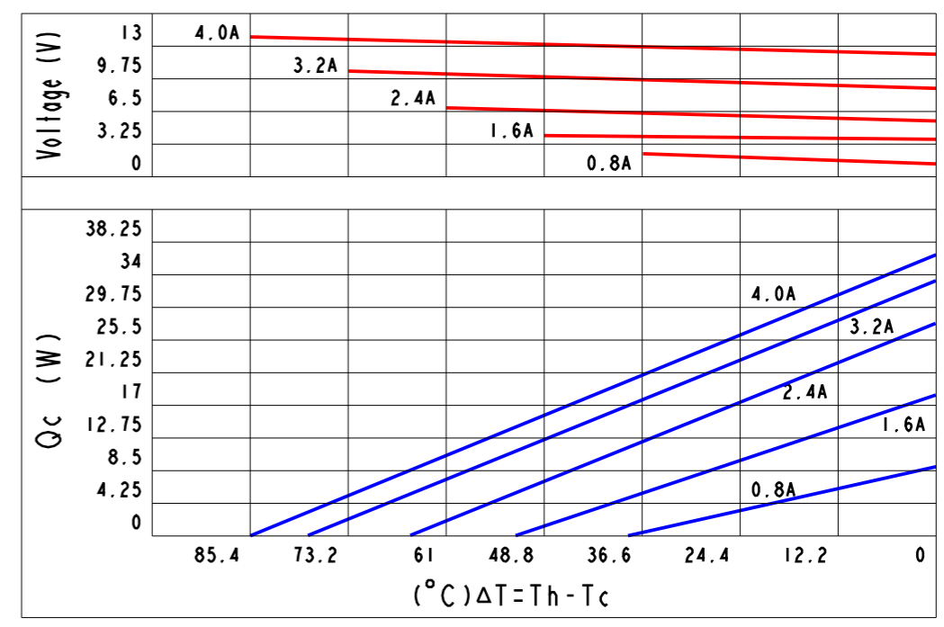
Curve Chart(Be Confined To TEC2-220043070):
