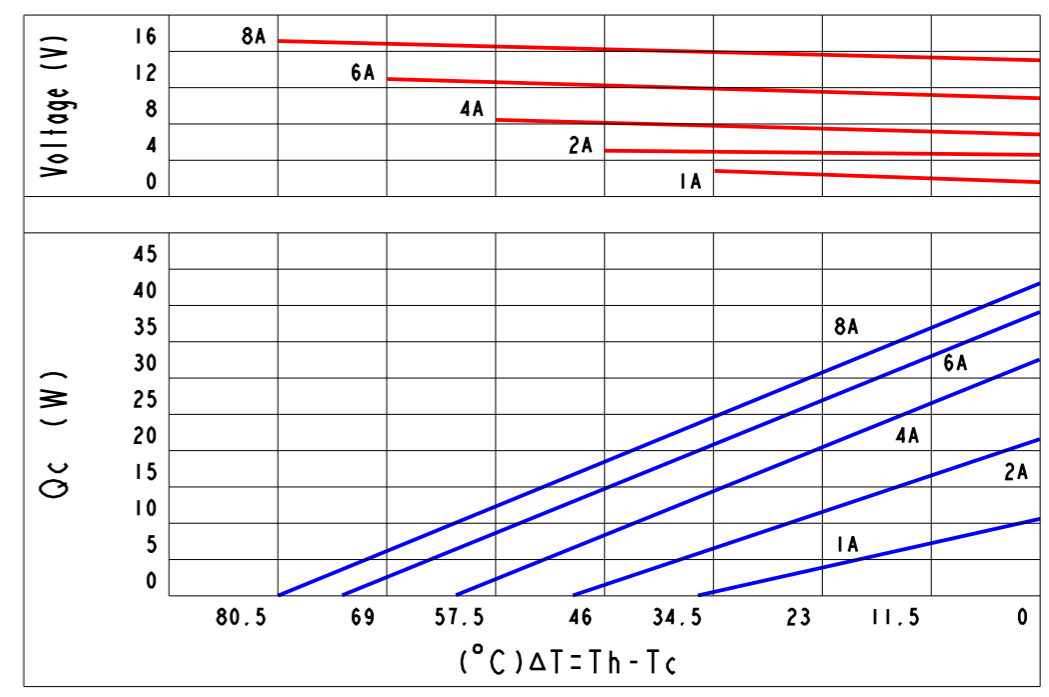
Curve Chart(Be Confined To TEC2-196084040):
