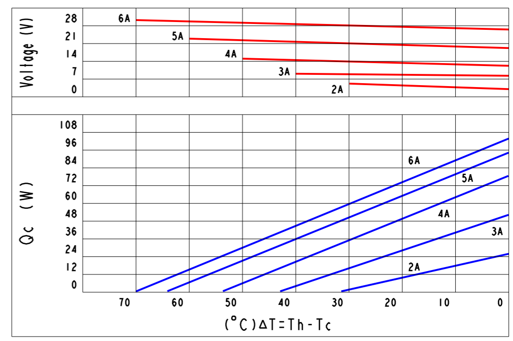
Curve Chart(Be Confined To TEC1-241064040):
