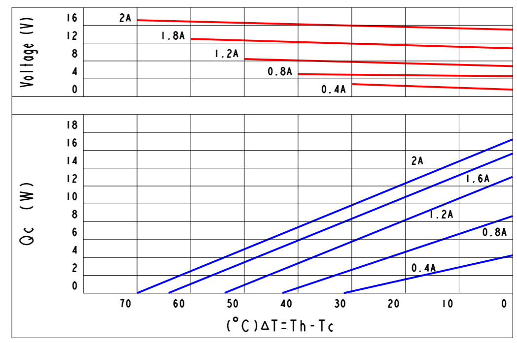
Curve Chart(Be Confined To TEC1-127202020):
