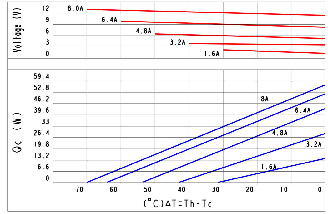
Curve Chart(Be Confined To TEC1-099082349):
