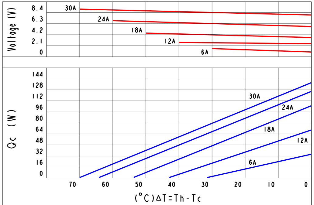
Curve Chart(Be Confined To TEC1-071304646):
